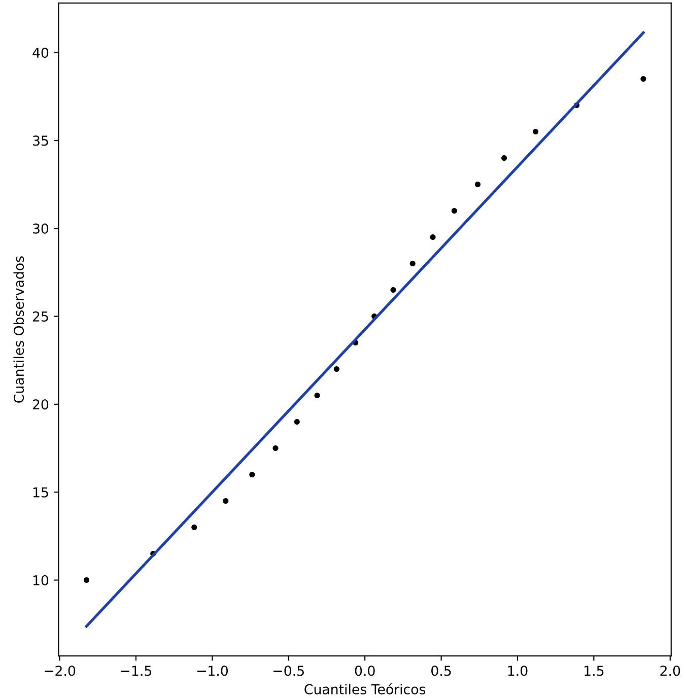
Q-Q Plot - Normal
